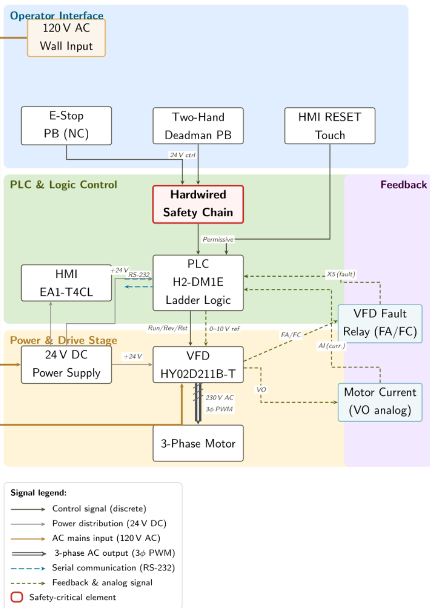
Figure 3: Control system block diagram — signal flow and functional domains.
